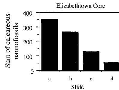
Figure 3: Histogram showing total number of calcareous nannofossil specimens tallied from 'a', 'b', 'c', and 'd' slides, Elizabethtown core. Note decreasing calcareous nannofossil numbers from 'a' slides (made on day of coring) to 'd' slides (made 222 days after coring)
