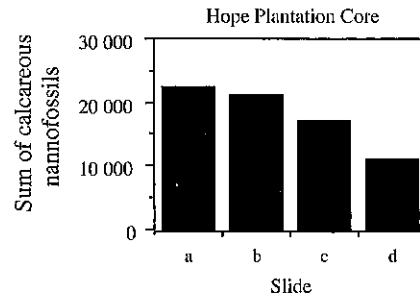
Figure 2: Histogram showing total number of calcareous nannofossil specimens tallied from 'a', 'b', 'c', and 'd' slides, Hope Plantation core. Note decreasing calcareous nannofossil numbers from 'a' slides (made on day of coring) to 'd' slides (made 222 days after coring)
