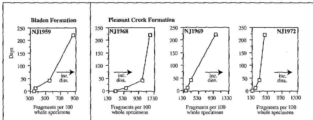
Figure 5: Plots of nannofossil fragments per 100 whole calcareous nannofossil specimens against number of days before slide preparation, Elizabethtown core. Note that increasing calcareous nannofossil dissolution is to the right (indicated by arrows). See Table 2 for depth of samples in core
