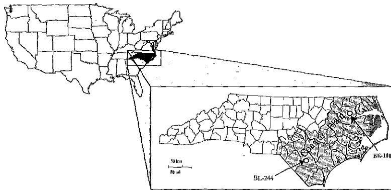
Figure 1: Map showing locations of the Hope Plantation (BE-110) and Elizabethtown (BL-244) Coreholes, North Carolina
